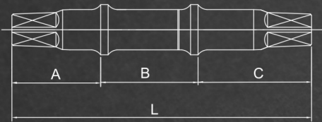
內牙中軸 Bolt Type Cotterless Axle
