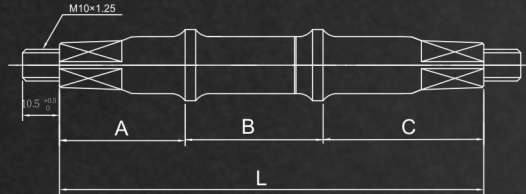
外牙中軸 Nut Type Cotterless Axle
